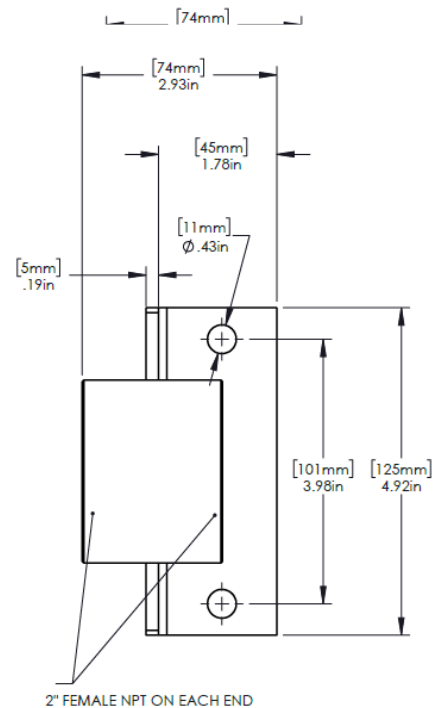
Standard 2" NPT Diesel Receiver
